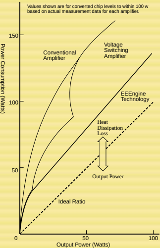
Power Consumption Comparison (f: 1KHz, RL: 4Ω)
