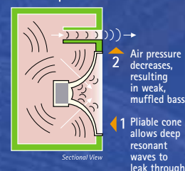
Standard Bass Reflex Speaker
