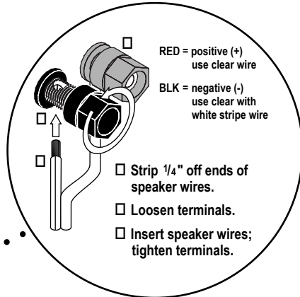
Speaker Wiring
