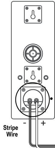
NS-A480 (Front Right Ch.)
