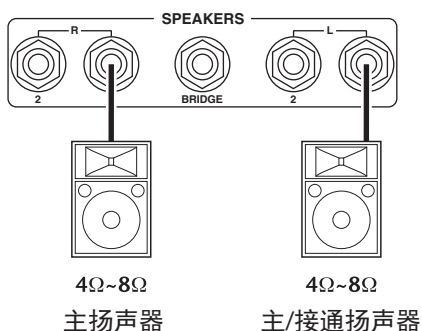
L/R接口上每次一根地连接
