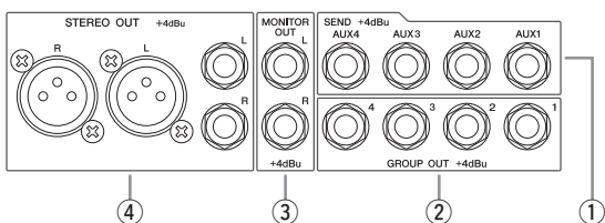
MG20XU Painel traseiro
