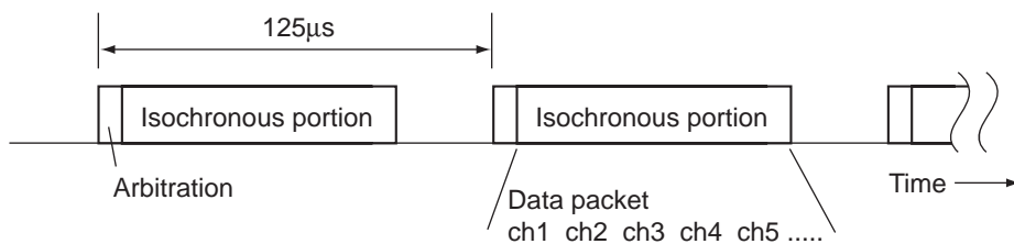
Figure 7: Isochronous sub-actions
