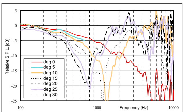
<Same enclosures, different power models>
